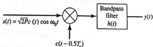
PROBLEM 3-17. Correlator illustrating spreading code self-noise.
